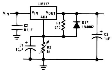
Figure 25. Adjustable Regulator with Improved Ripple Rejection
