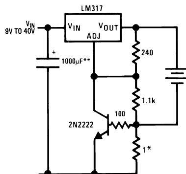
Figure 44. Current Limited 6V Charger
