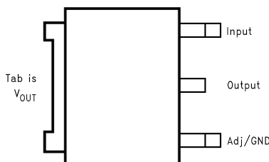
Figure 10. TO-252 (MDT)
