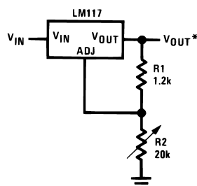
Figure 32. 1.2V–20V Regulator with Minimum Program Current
