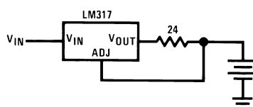
Figure 42. 50mA Constant Current Battery Charger
