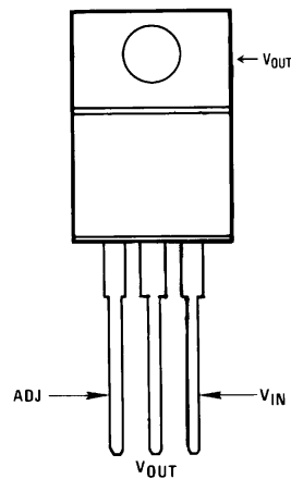
Figure 6. TO-220 (T) Plastic Package
