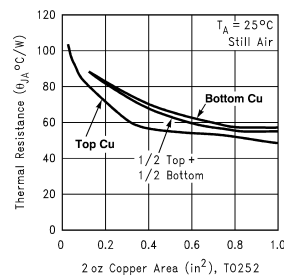
Figure 18. \theta_{JA} vs 2oz Copper Area for TO-252
